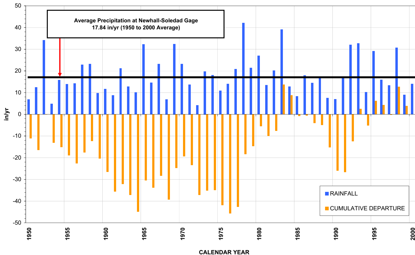
FIGURE 2-5 ANNUAL PRECIPITATION AND CUMULATIVE DEPARTURE FROM THE 1950 THROUGH 2000 AVERAGE AT THE NEWHALL-SOLEDAD RAIN GAGE
