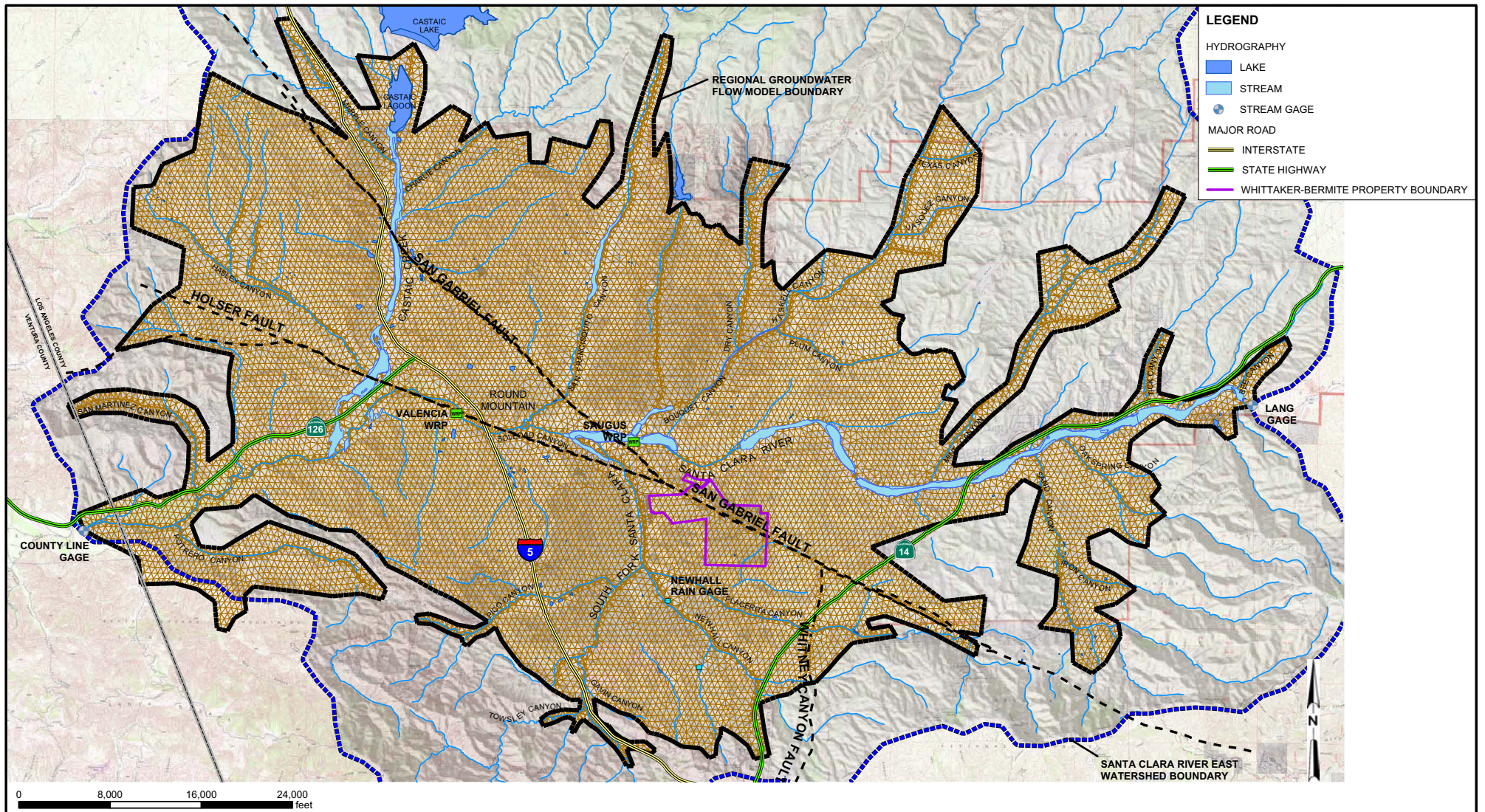
FIGURE 2-5 REGIONAL MODEL GRID ANALYSIS OF PERCHLORATE CONTAINMENT IN GROUNDWATER NEAR THE WHITTAKER-BERMITE PROPERTY SANTA CLARITA, CALIFORNIA
