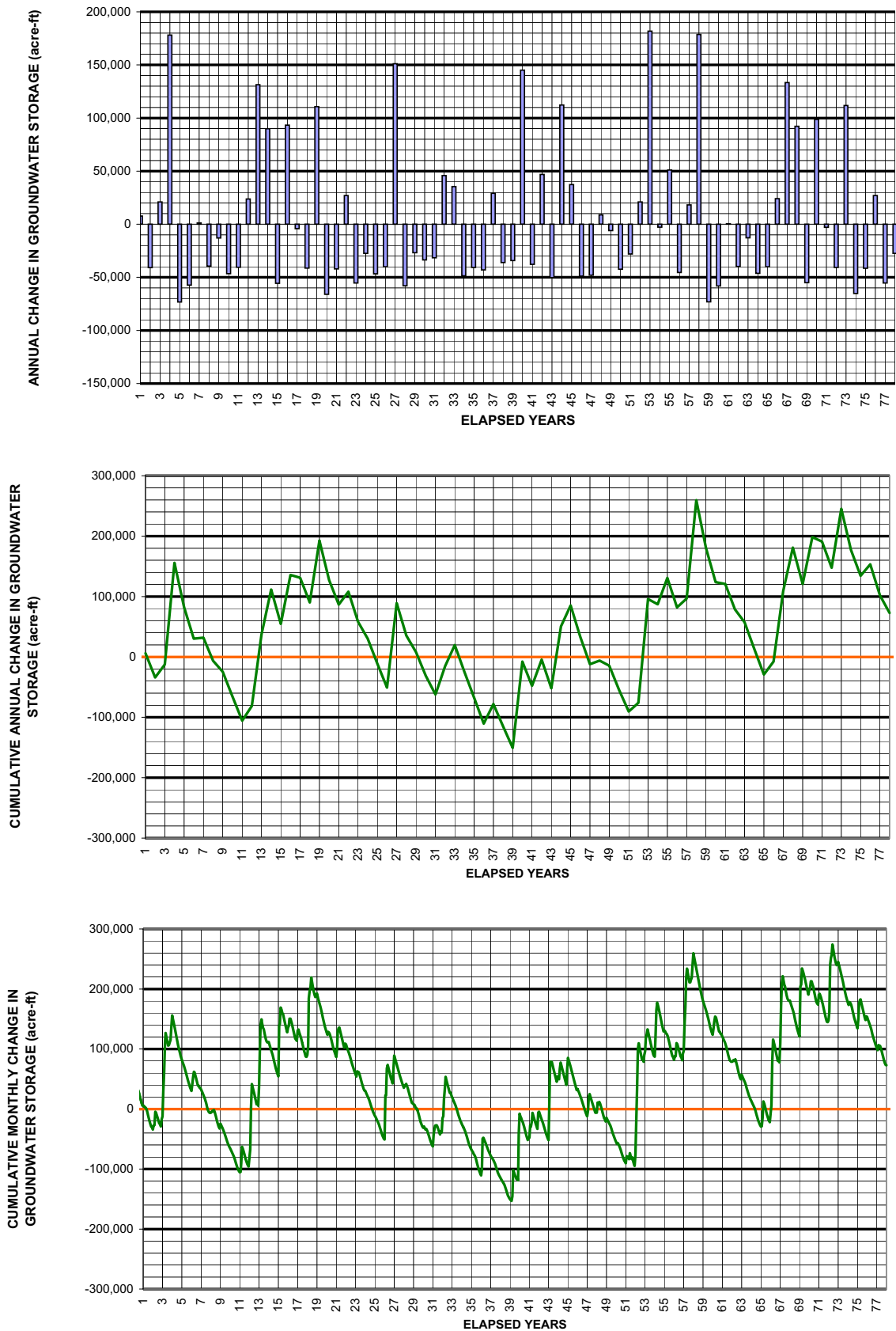
FIGURE ES-7 ANNUAL CHANGE AND CUMULATIVE CHANGE IN GROUNDWATER STORAGE ANALYSIS OF PERCHLORATE CONTAMINANT IN GROUNDWATER NEAR THE WHITTAKER-BERMITE PROPERTY SANTA CLARITA, CALIFORNIA
