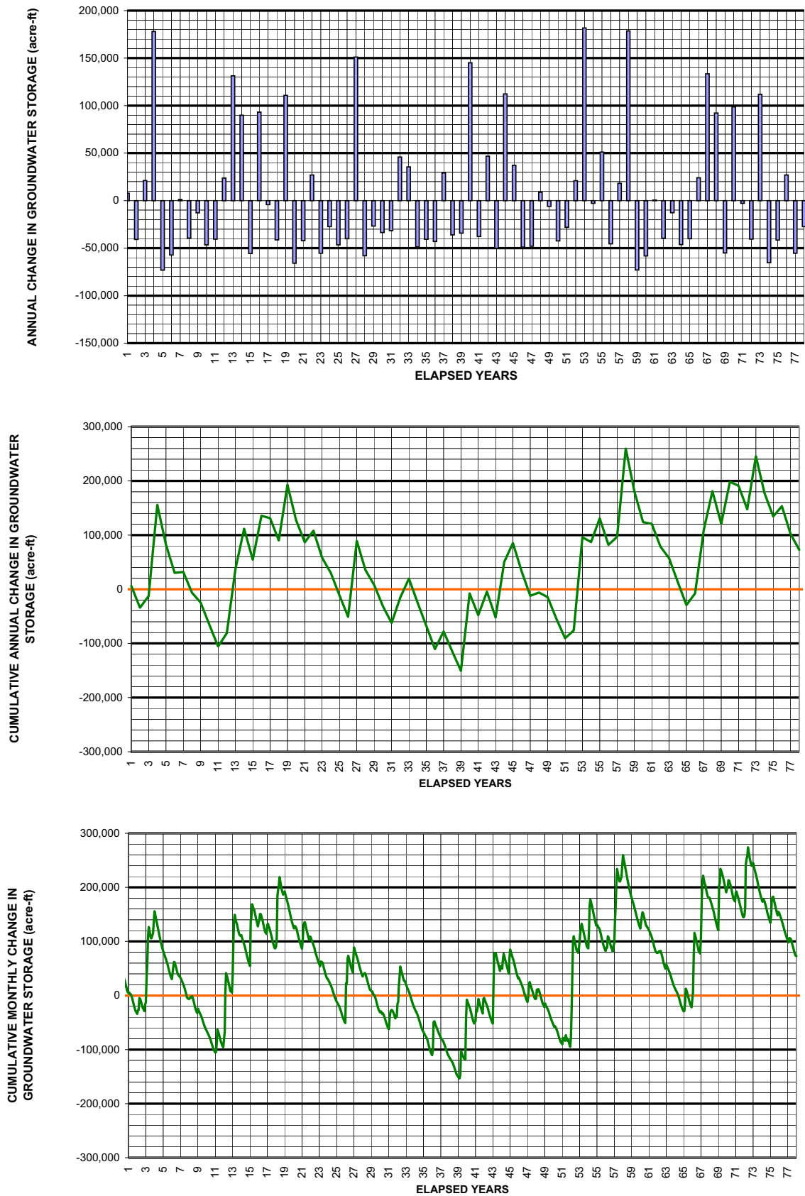
FIGURE 2-21 ANNUAL CHANGE AND CUMULATIVE CHANGE IN GROUNDWATER STORAGE ANALYSIS OF PERCHLORATE CONTAMINANT IN GROUNDWATER NEAR THE WHITTAKER-BERMITE PROPERTY SANTA CLARITA, CALIFORNIA
