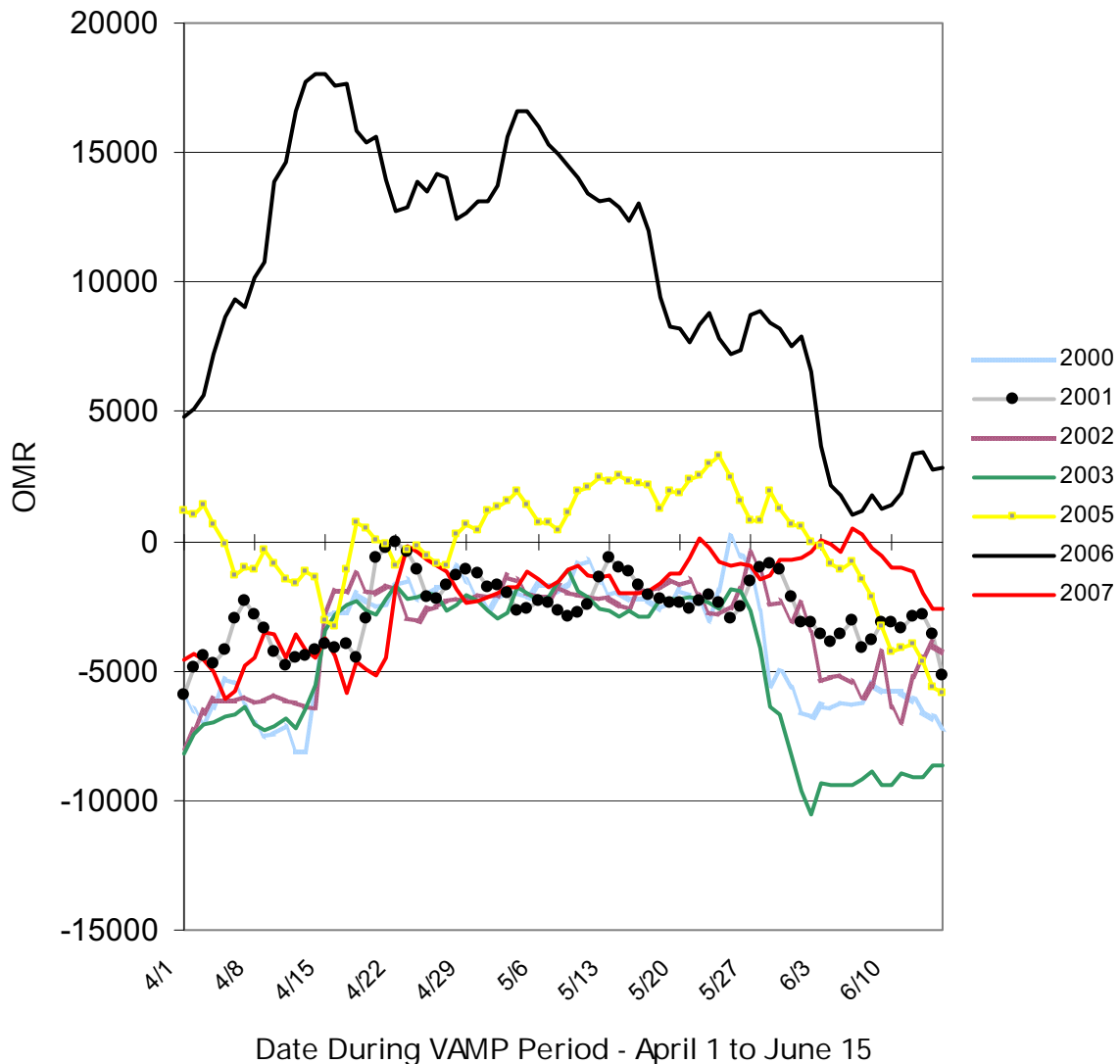
Figure B-15. OMR flows across VAMP period (usually April 15-May 15). Note that although exact VAMP conditions vary across years, the period is easily identified by OMR flows no more negative than -2000 cfs.
