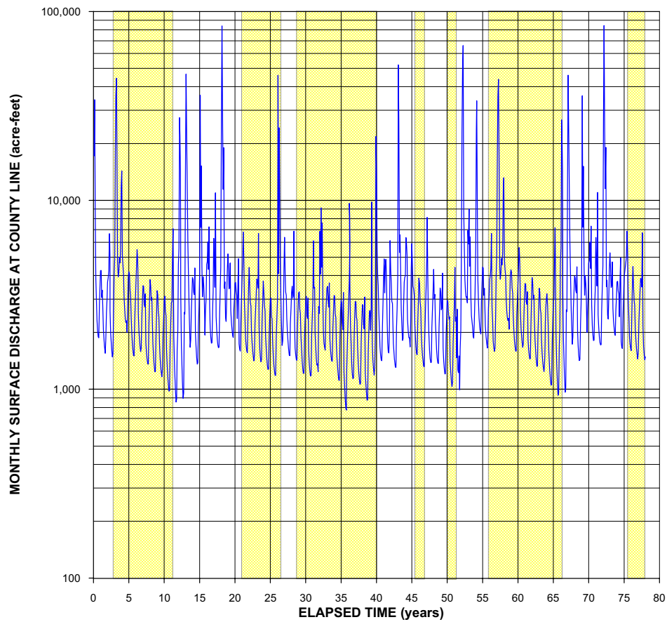
FIGURE 4-11 SIMULATED SANTA CLARA RIVER FLOW AT COUNTY LINE
