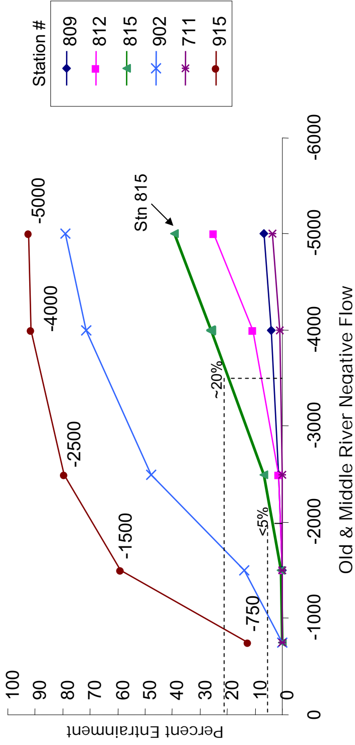
Figure B-16: Pump Entrainment at Various Levels of Negative Flow at Old and Middle River Monitoring
