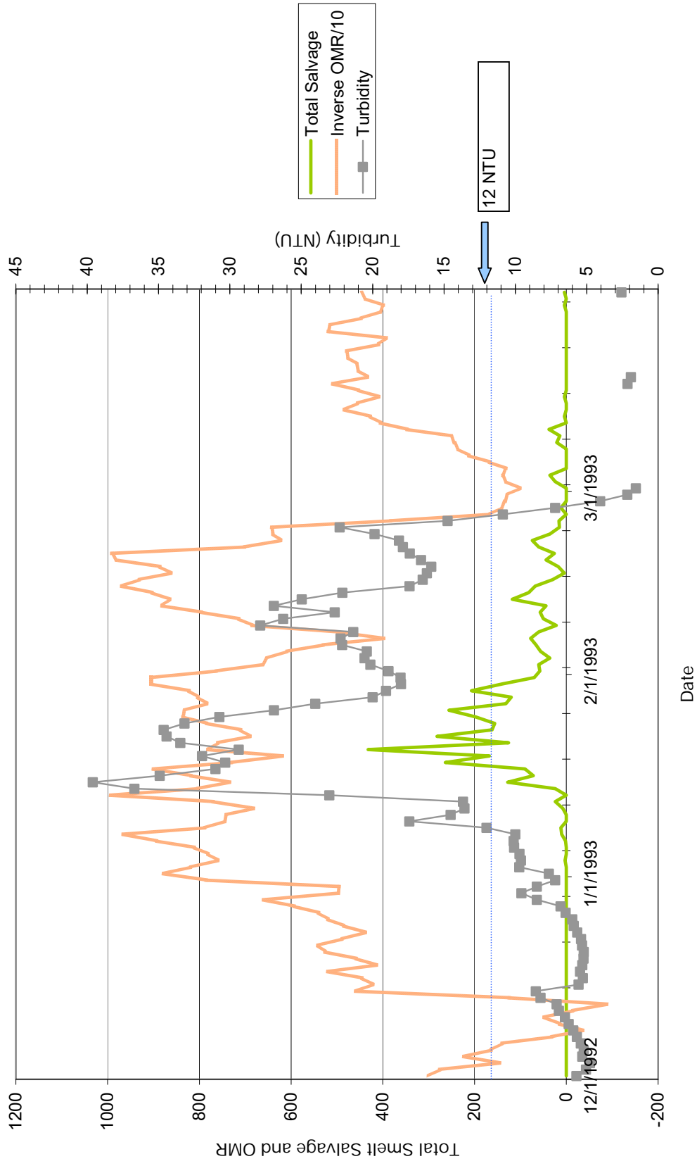
Figure B-3: 1993 WY OMR, Turbidity, Salvage
