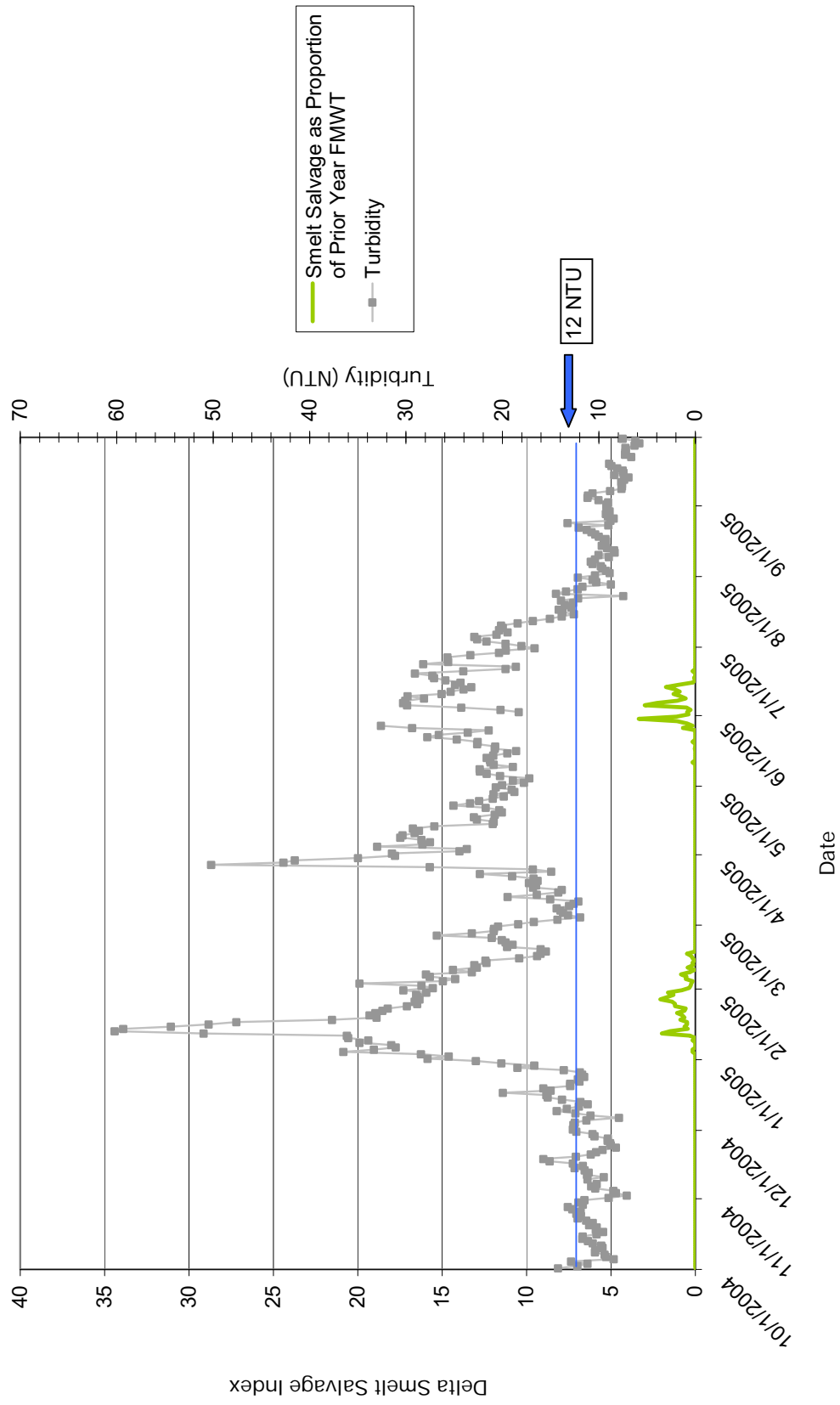
Figure B-10: 2005 WY Salvage Index
