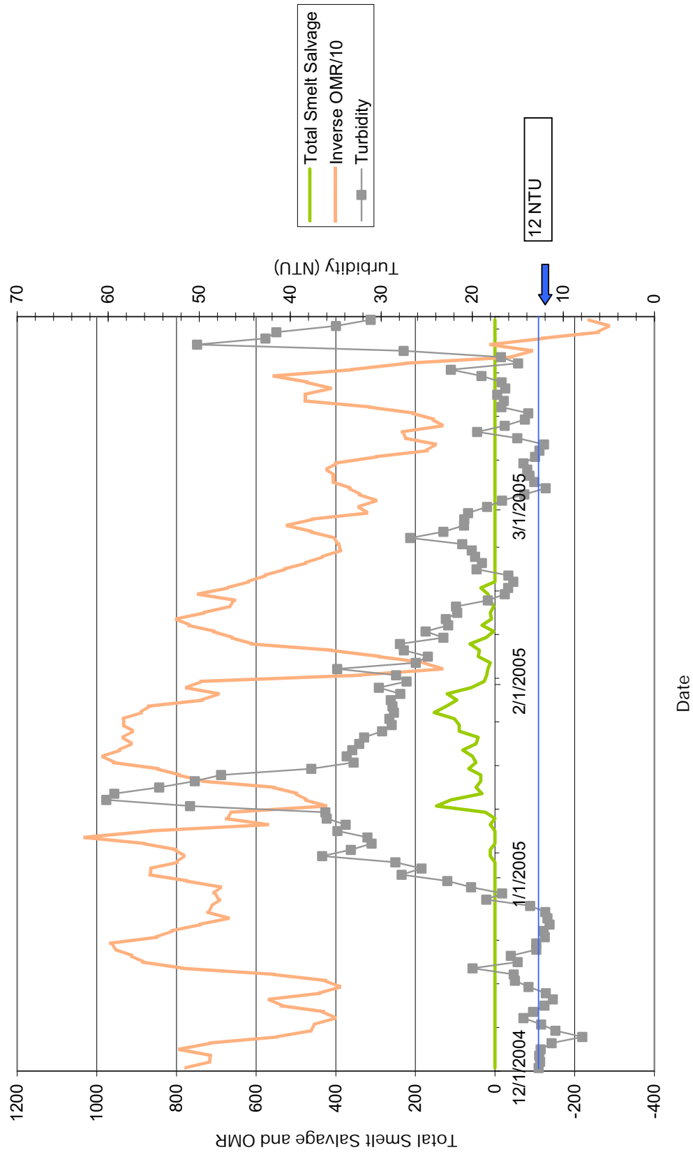
Figure B-6: 2005 WY OMR, Turbidity, Salvage
