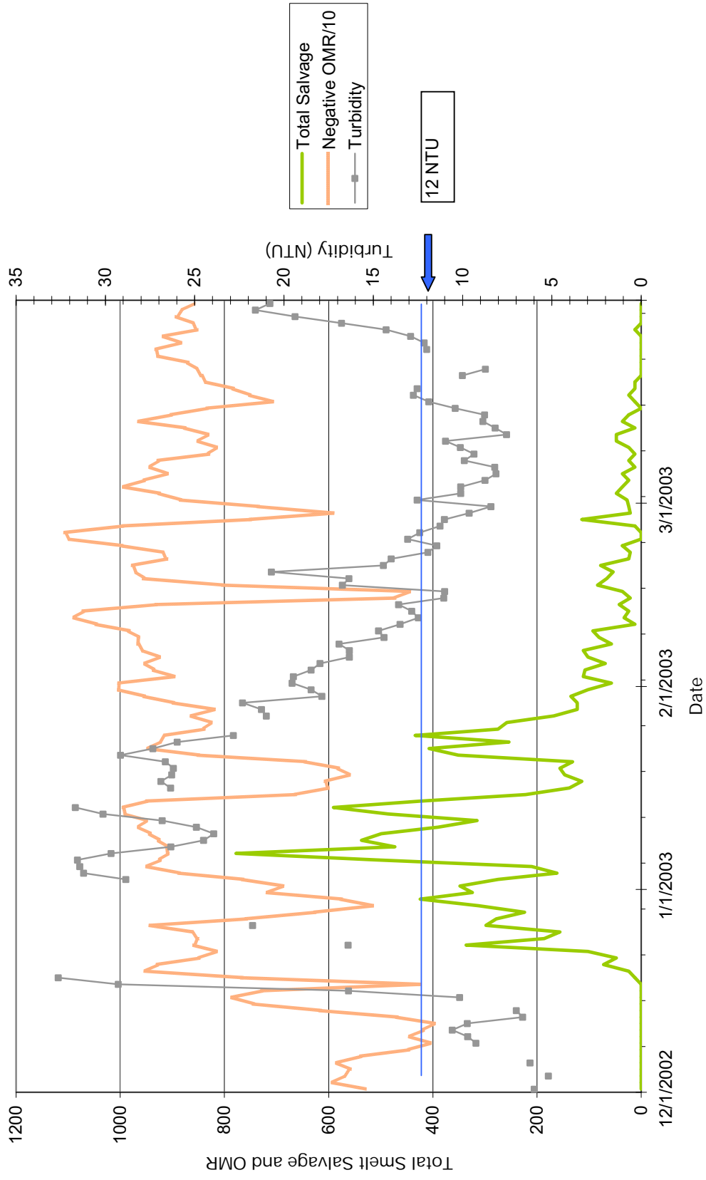
Figure B-4: 2003 WY OMR, Turbidity, Salvage
